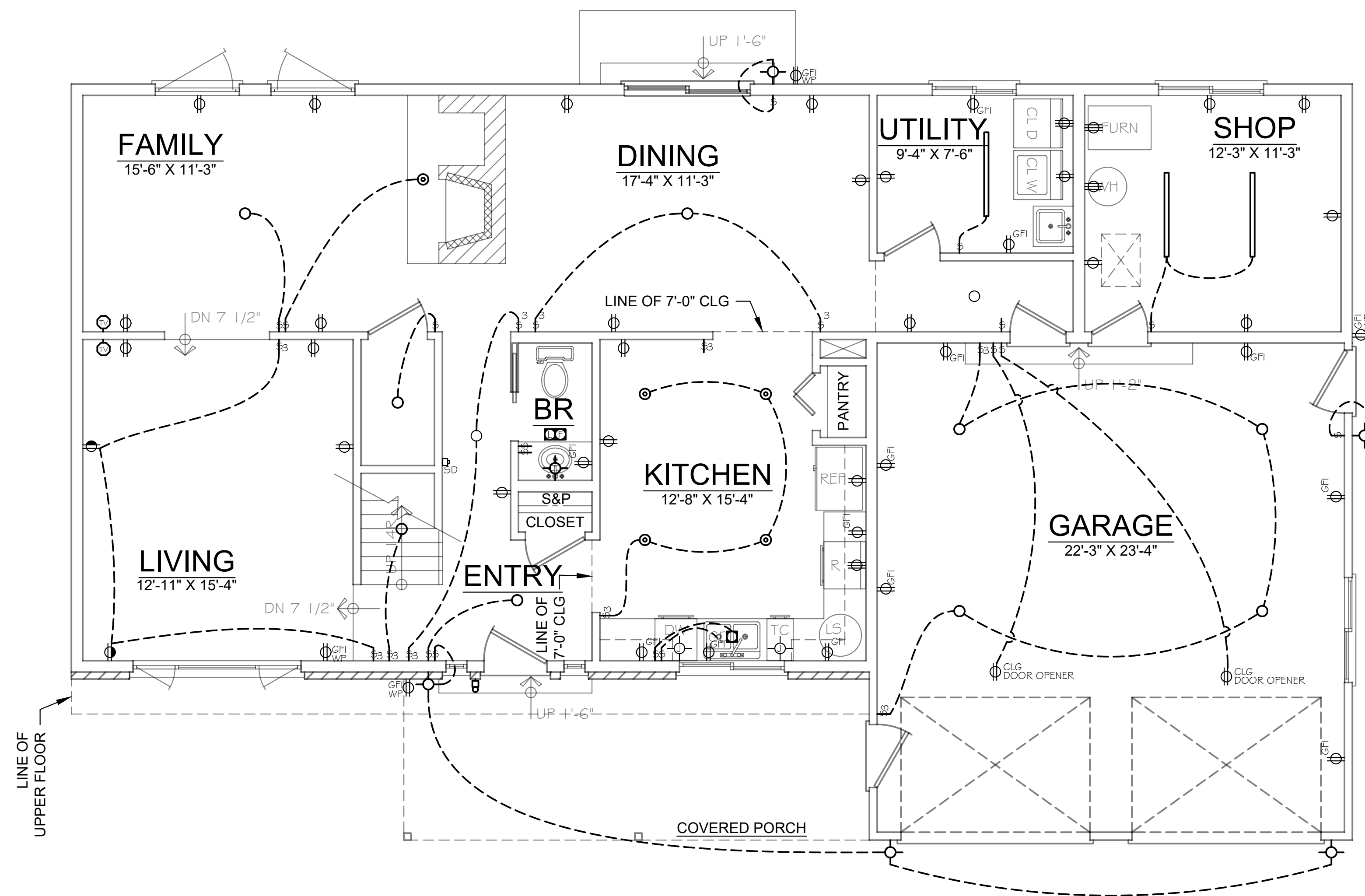
MAIN FLOOR ELECTRICAL SCALE: 1/4" = 1'-0"
